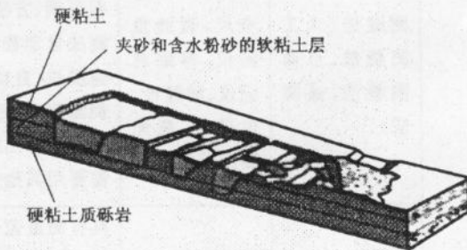
(f) 侧向扩展(Lateral spread)
