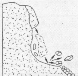
(a) 崩落(Falls)
