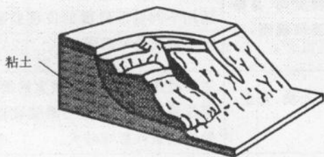
(c) 滑动(Slide)
